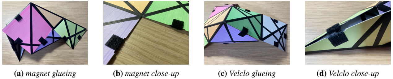
Figure 1: glueing mechanism at foldings made by magnet or velcro.
