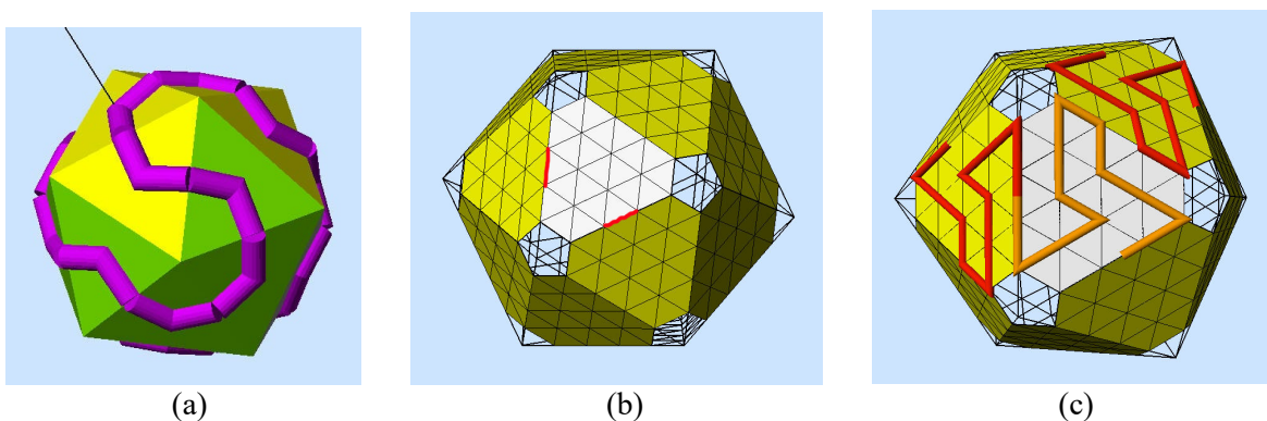
Figure 9: (a) a Hamiltonian path; (b) subdivided icosahedron faces; (c) a possible Gopher pattern.
