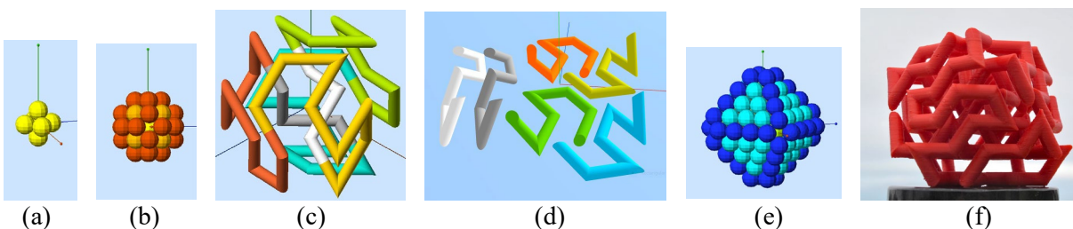
Figure 8: (a) Octahedral core, 6 atoms; (b) 2 nd shell, 32 atoms. (c) Path of the 2-level Gopher-Onion; (d) assembly based on six parts. (e) 3 rd shell, 102 atoms; (f) a 3-level Gopher-Onion sculpture.
