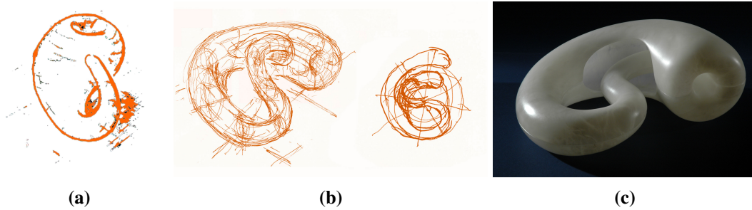
Figure 2: Giorgini's drawings of (a) the Klein bottle, and (b) the Klein bottle with a disk removed around the self-intersection of the surface; (c) Giorgini's sculpture of the Klein bottle minus a disk: Modified Klein; width: 20 inches; height: 6 inches; material: alabaster.
