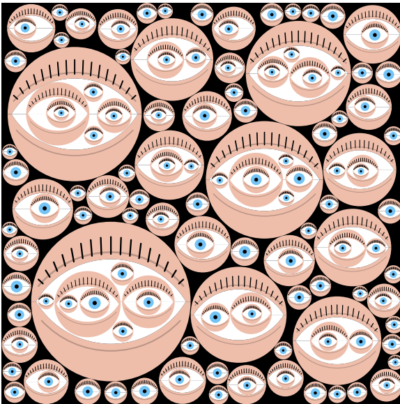
Figure 6: A pattern with hollow eye motifs, with 150 eyes, c=1.20 , N=3 , and 56% fill.
