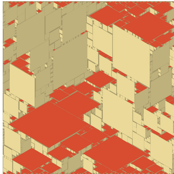
Figure 7: A pattern of three rhombi, 250 of each orientation, with c=1.52 , N=8 , and 91% fill.
