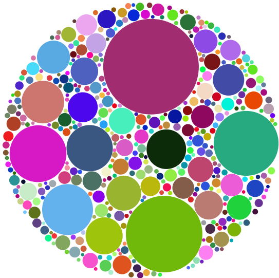
Figure 4: A pattern of 401 circles, with parameters c=1.32 , N=2.5 , 81.62% fill, and 37161 trials.
