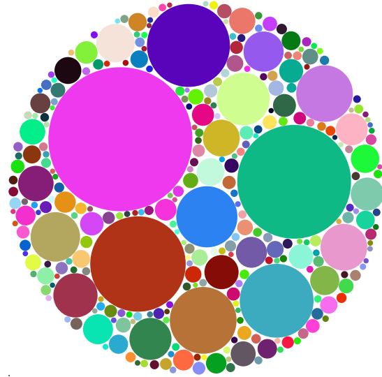
Figure 3: A pattern of 299 circles, with parameters c=1.40 , N=2.5 , 86.47% fill, and 178239 trials.
