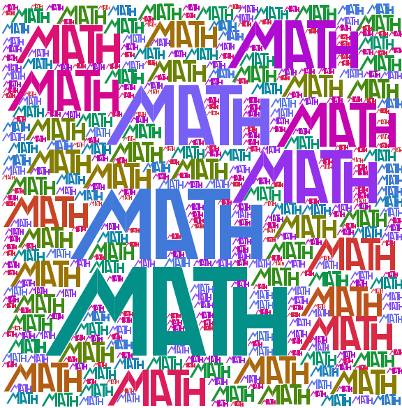
Figure 10: A pattern made from the word MATH , with 400 copies, c=1.126 , N=2 , and 50% fill.
