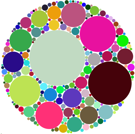
Figure 2: A pattern of 231 circles, with parameters c=1.48 , N=2.5 , 89.74% fill, and 2973700 trials.
