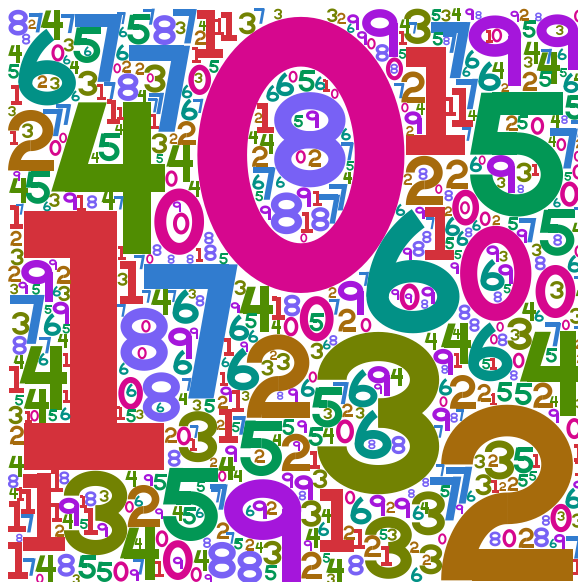
Figure 9: A sequence of 600 digit motifs 0-9, with c=1.19 , N=2 , and 68% fill.
