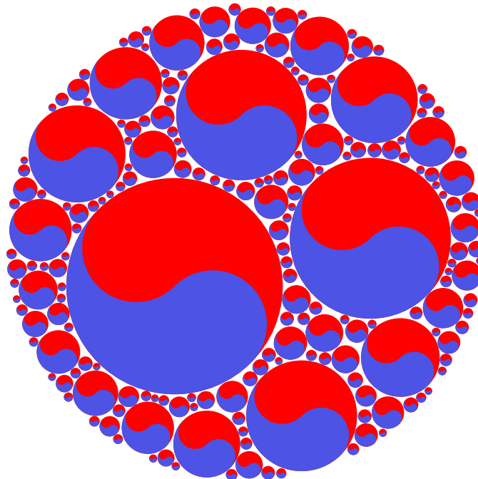
Figure 1: A random circle fractal with yin-yang motifs, with 200 motifs, c=1.46 , N=2 , 89% fill.
