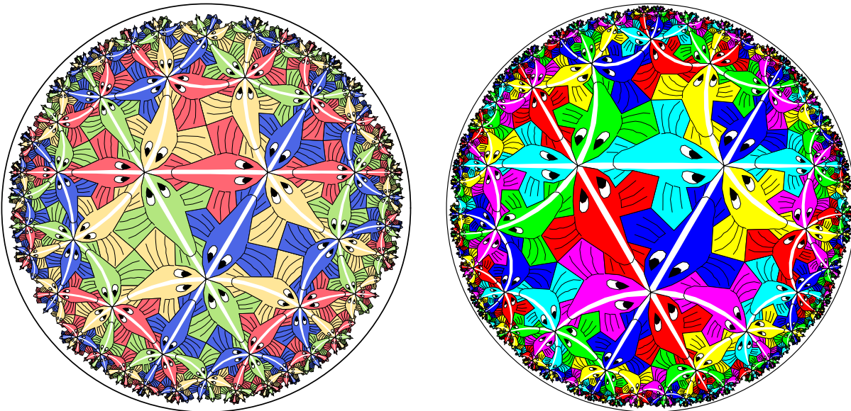
Figure 11: A (3,4,3) pattern related to Escher's Circle Limit III .
