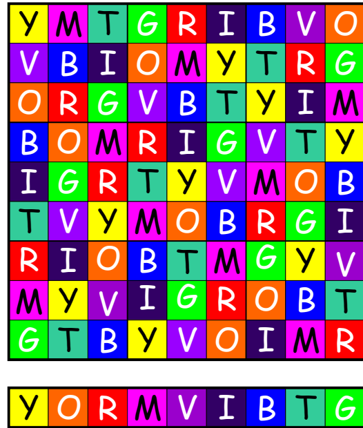
Figure 9: The solution, using the 9 colours
