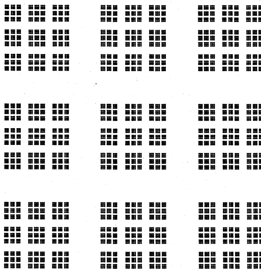
Figure 2: A simple recursive set of squares, five levels deep.
