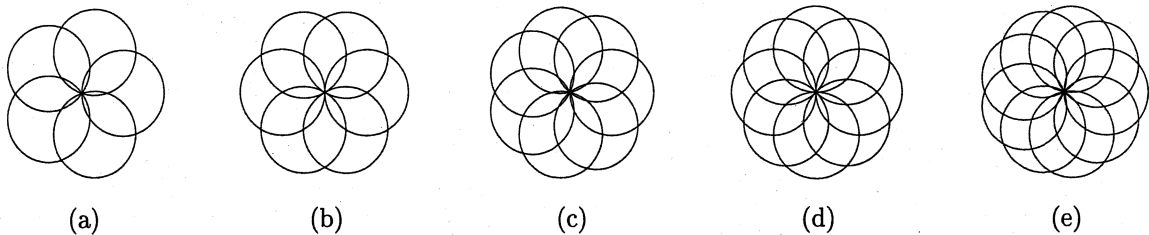
Figure 7: Rosettes with 5 to 9 circles
