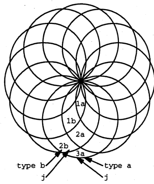
Figure 6: Notation for slots in the rosette
