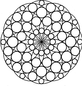
Figure 8: Circles inscribed in the rosette
