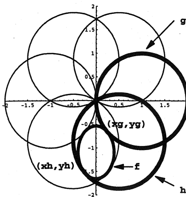
Figure 4: A circular rosette containing n = 6 circles. An ellipse ( f ) is shown tangent to two adjacent circles ( g and h ). Also indicated are the two contact points (x_g, y_g) and (x_h, y_h) .
