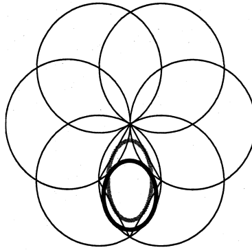
Figure 12: The maximum area inscribed ellipses for both a circular and polygonal rosette.
