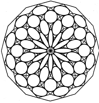
Figure 11: Maximum area ellipses inscribed in the polygonal approximation of the rosette
