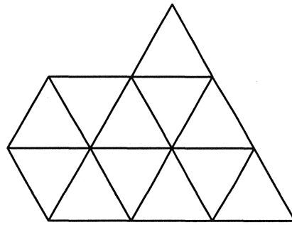
Figure 6: Configuration containing a total of seventeen triangles
