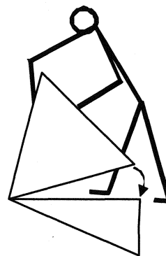
Figure 1: Comparing to a reference triangle
