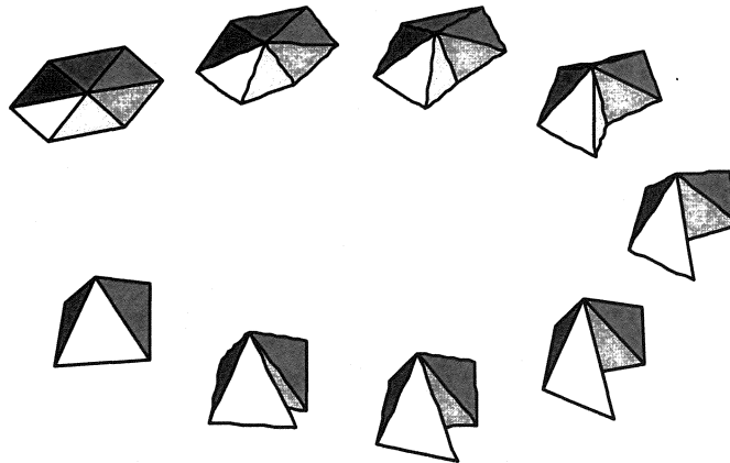
Figure 3: Folding and tucking two triangles
