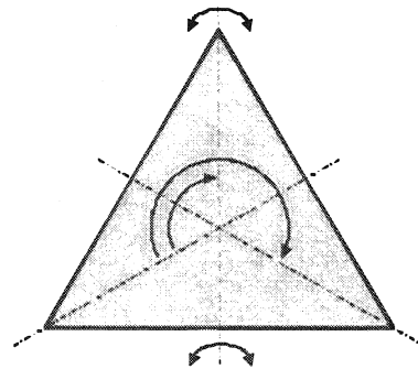
Figure 9: Some symmetries of the triangle
