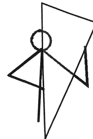
Figure 10: The line of reflection of the face
