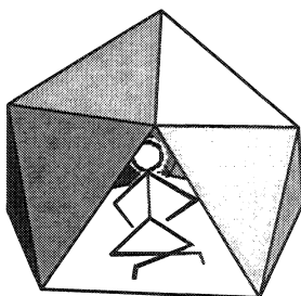
Figure 4: The partial icosahedron
