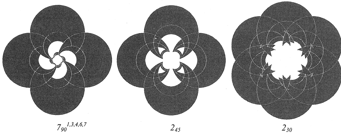
Figure 7: Spiroilateral inversions
