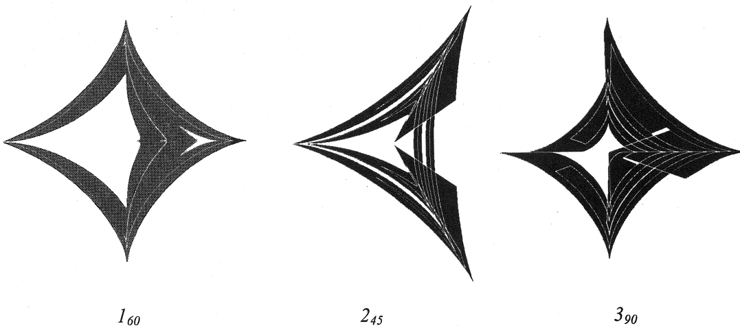
Figure 14: Hypocycloid spirolaterals
