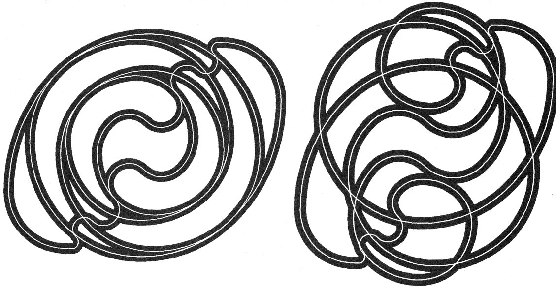
Figure 5: Curved spirolaterals of 14 90
