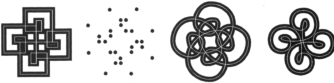
Figure 4: Curved spirolateral 7 90
