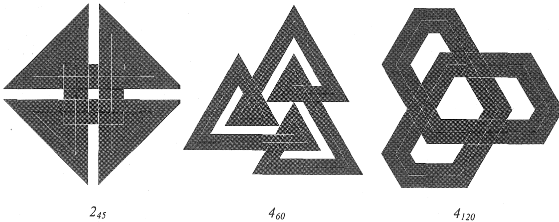
Figure 1: Closed spirolaterals
