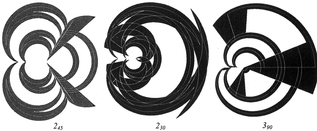
Figure 15: Epicycloid spirolaterals
