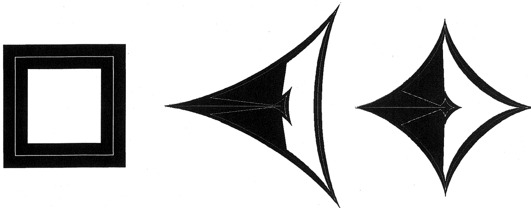
Figure 12: Hypocycloid spirolateral 1_90
