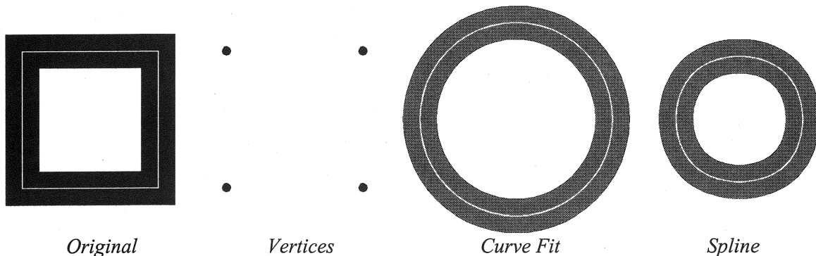
Figure 3: Curved spirolateral 1_{90}
