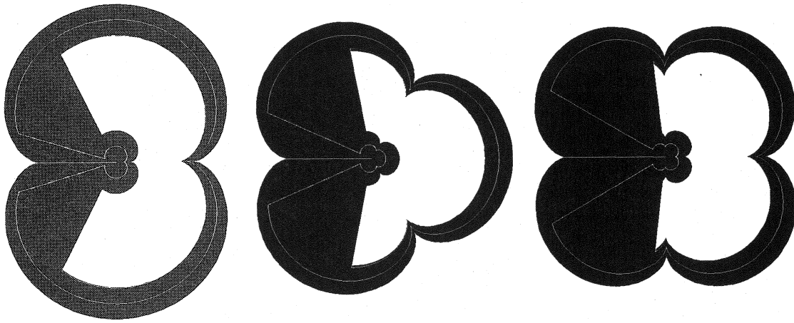
Figure 13: Epicycloid spiroilateral 1 90
