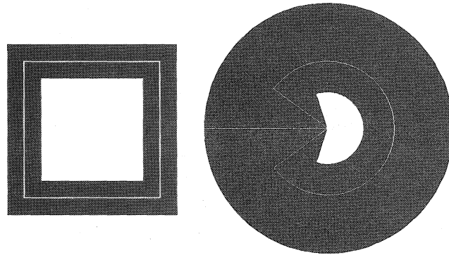
Figure 8: antiMercator spiroilateral 1 90
