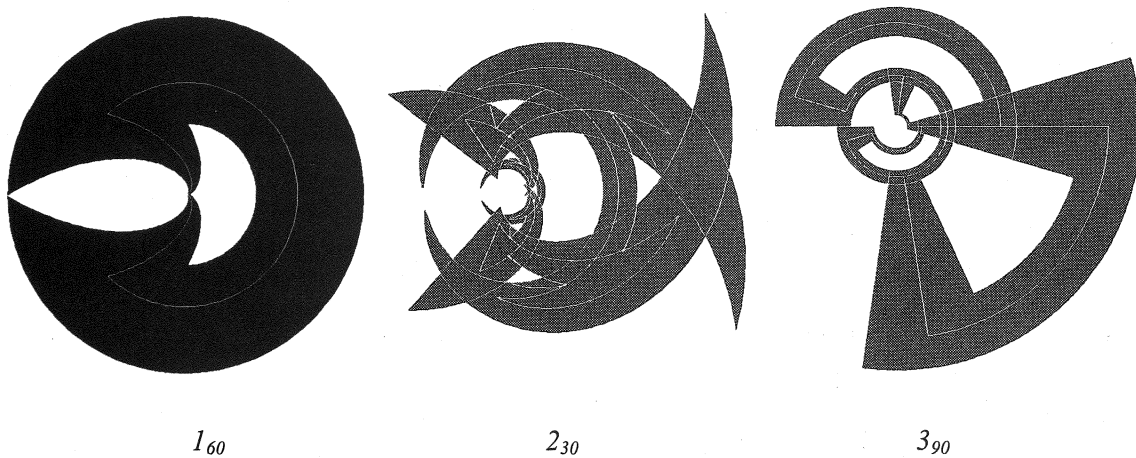
Figure 9: antiMercator spiroilaterals
