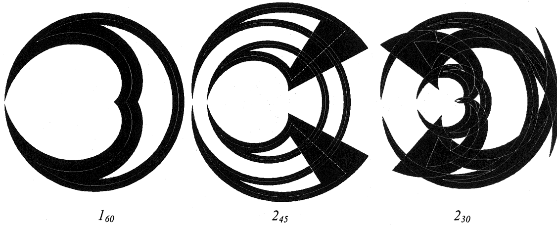
Figure 11: Circular spiroilaterals
