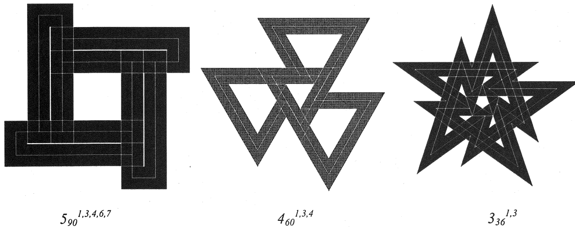
Figure 2: Closed spirolaterals with reversals
