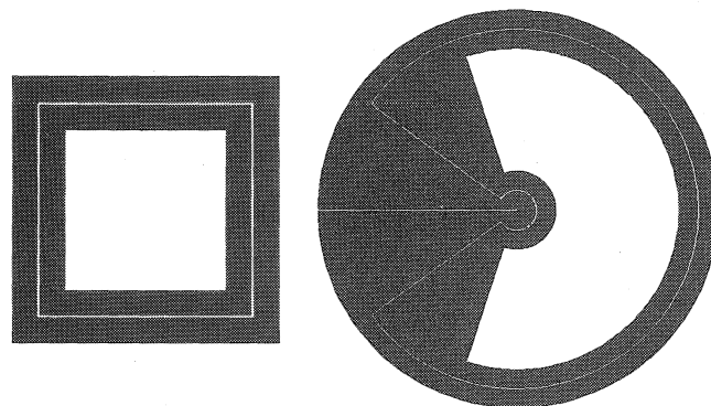
Figure 10: Circular spiroilateral 1 90
