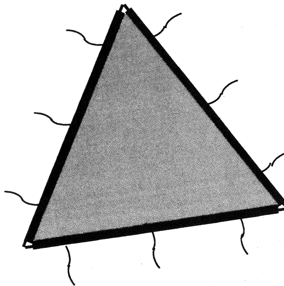
Figure 2 A triangle
