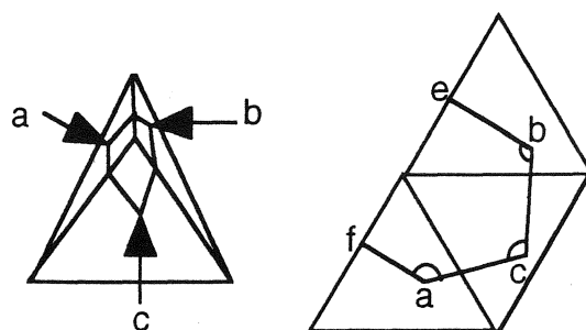
Figure 6 Tetrahedron with a geodesic triangle 'abc' (left) becomes pentagon 'facbe' after the enclosed tetrahedral vertex is opened up by untying (right).
